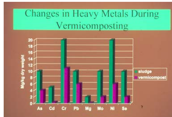
Figure 22. Changes in heavy metals during vermicomposting
