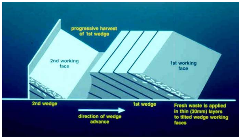
Figure 3. The Wedge Vermicomposting System
