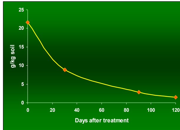
Figure 23. Breakdown of polycyclic aromatic hydrocarbons after a polluted soil treatment with cattle vermicompost (61.9m 3 /ha) and vermicompost teas (9.23l/ha)
